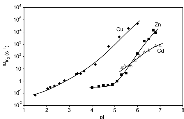
Figure 4. The pH dependence of the second-order rate constant {}^{\text{fM}}k_2 for the formation of the \text{H}_4\text{L}^3 complexes. The curves show the best results of fitting by Equation (1) for (a) \text{Cu}^{\text{II}} (full diamonds) and (c) \text{Cd}^{\text{II}} (empty triangles) and (b) fitting by Equation (2) for \text{Zn}^{\text{II}} (full squares).
