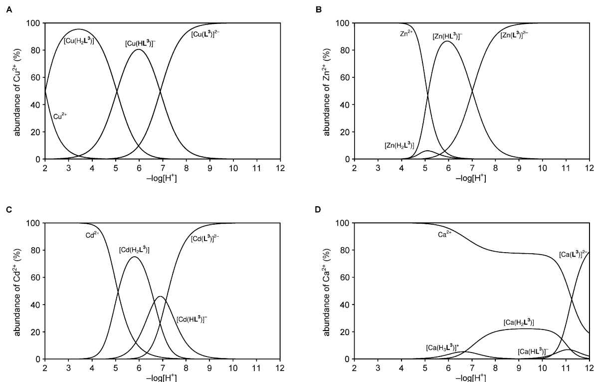
Figure 3. Distribution diagrams of metal-containing species in the M^{II} – H_4L^3 systems with c_L = c_M = 0.004 M for M^{II} = Cu^{II} (A), Zn^{II} (B) and Cd^{II} (C) and Ca^{II} (D).
