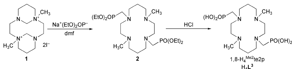
Scheme 2. Novel approach in ligand synthesis.
