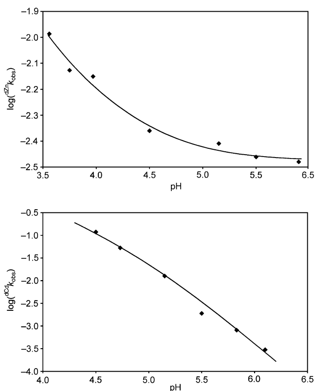
Figure 6. Dependence of dissociation rate constants of zinc(II) and cadmium(II) complexes with H_4L^3 on pH. The curves show the best fits according to Equation (4).
