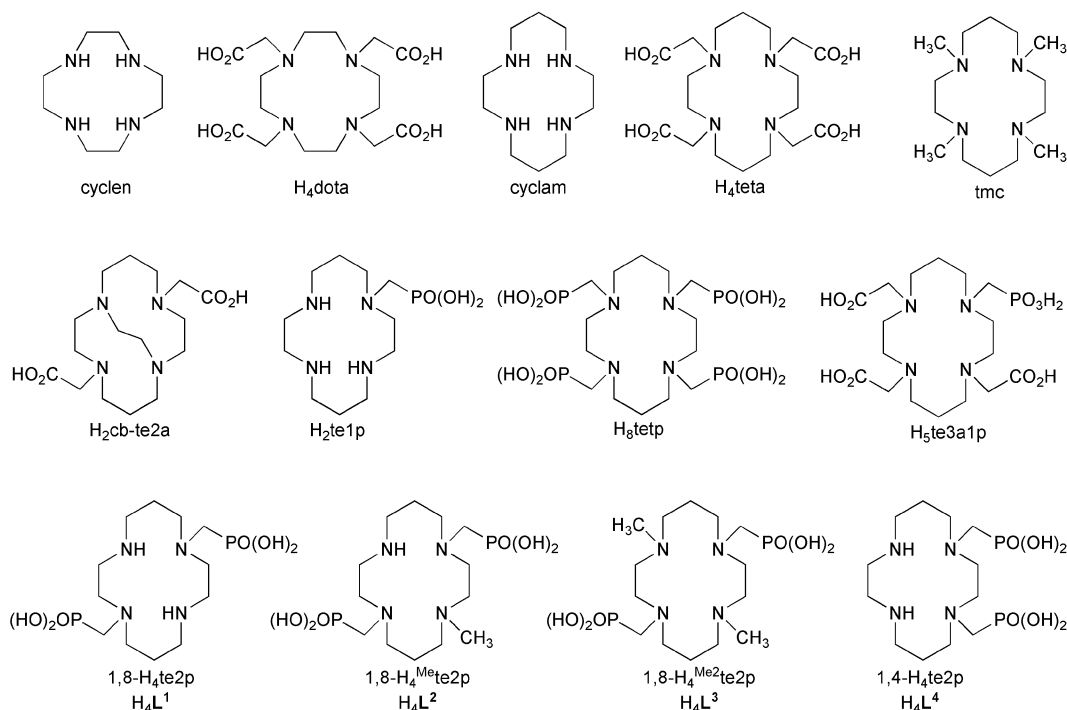
Scheme 1. Structures of ligands mentioned in the text.
