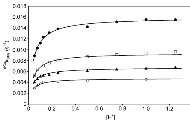
Figure 5. Dependence of the dissociation rate constants of the \text{Cu}^{\text{II}} – \text{H}_4\text{L}^3 complex on proton concentration and temperature. 20 °C – open diamonds; 25 °C – full triangles; 30 °C – open squares; 35 °C – full circles. The lines correspond to the best fits according to Equation (3).
