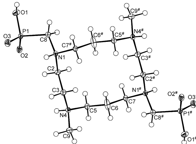
Figure 1. Structure of centrosymmetric molecular cation (H_6L^3)^{2+} found in the structure of (H_6L^3)Cl_2 \cdot 4H_2O . Thermal ellipsoids show 60% probability level.
