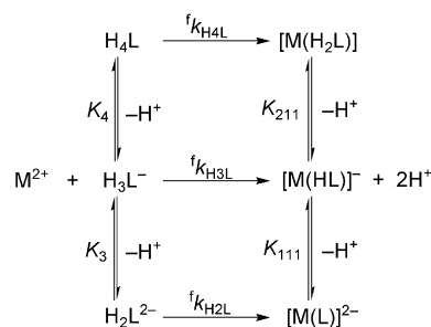
Scheme 3. General mechanism of complex formation.
