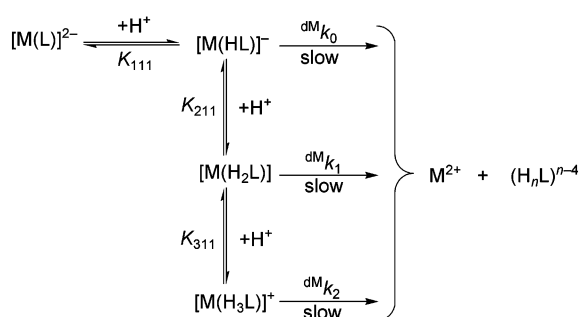
Scheme 5. The reaction mechanism proposed for dissociation of the zinc(II) and cadmium(II) complexes with H_4L^3 .
