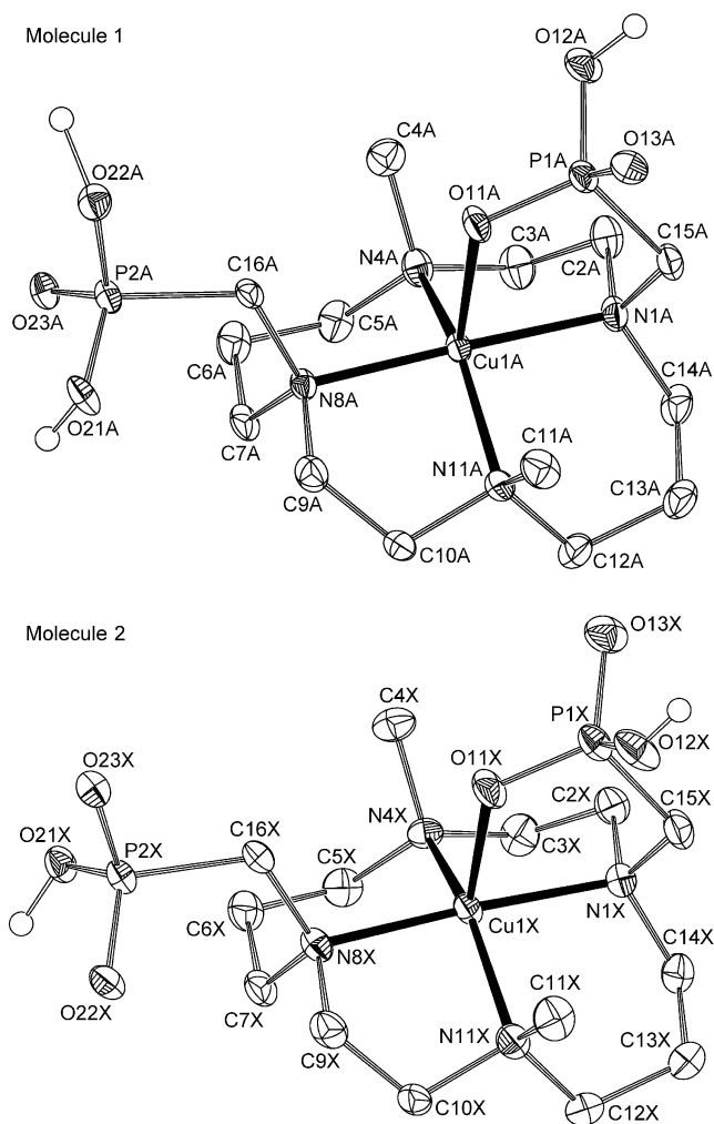
Figure 2. Structure of complex units, [\text{Cu}(\text{H}_3\text{L}^3)]^+ (molecule 1) and [\text{Cu}(\text{H}_2\text{L}^3)] (molecule 2), found in the structure of [\text{Cu}(\text{H}_3\text{L}^3)][\text{Cu}(\text{H}_2\text{L}^3)]\text{PF}_6 \cdot 3\text{H}_2\text{O} . The hydrogen atoms attached to the carbon atoms are omitted for the sake of clarity. Thermal ellipsoids show 60% probability level.
